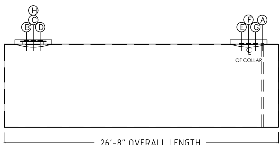
ELEVATION VIEW
