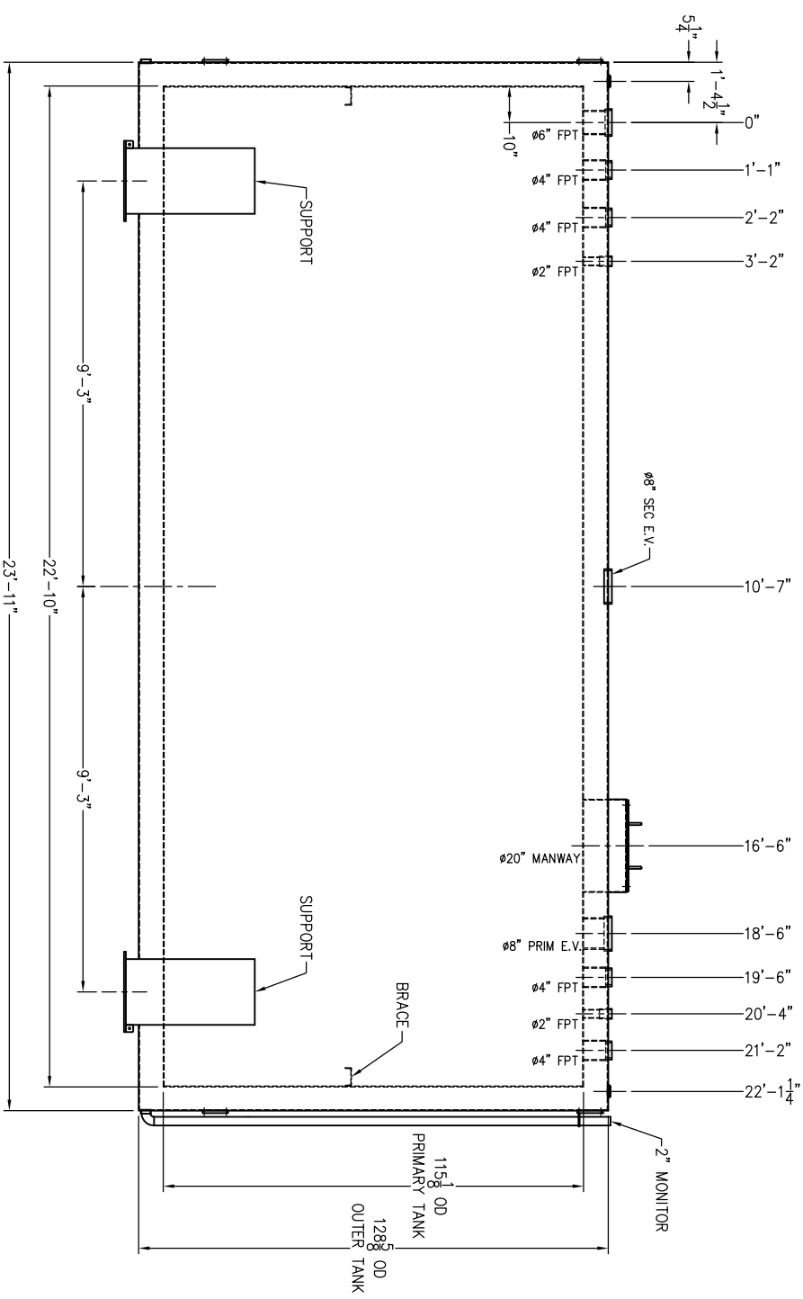
ELEVATION VIEW
